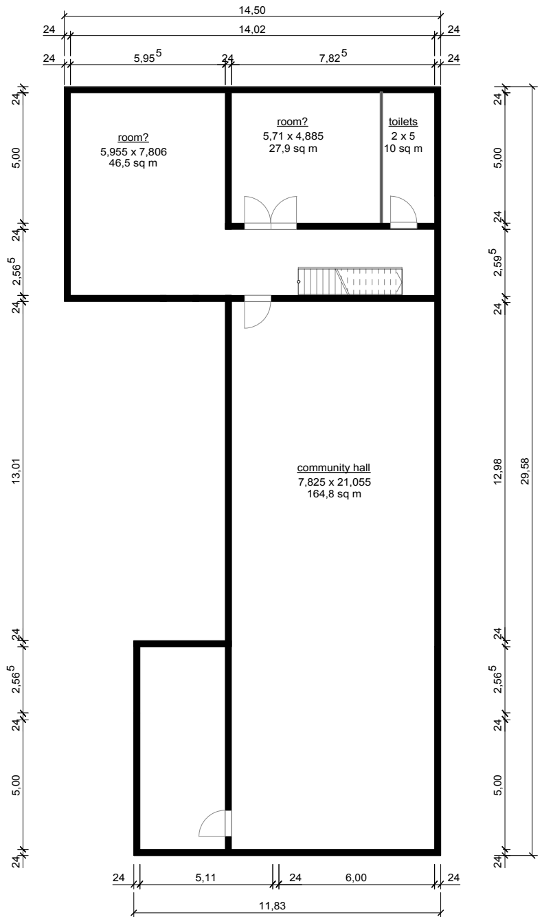
basement floor 1:200
