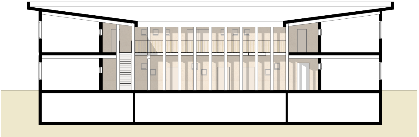
section A 1:200
