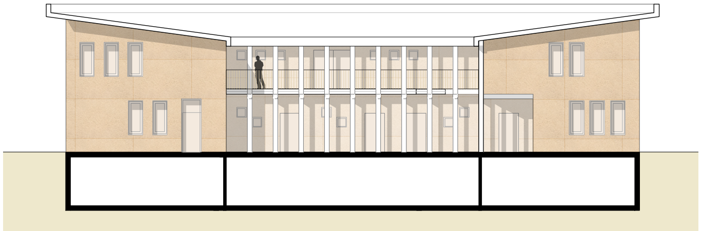
west elevation 1:200
