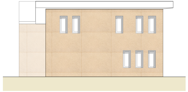
south elevation 1:200
